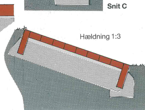
Snit C
